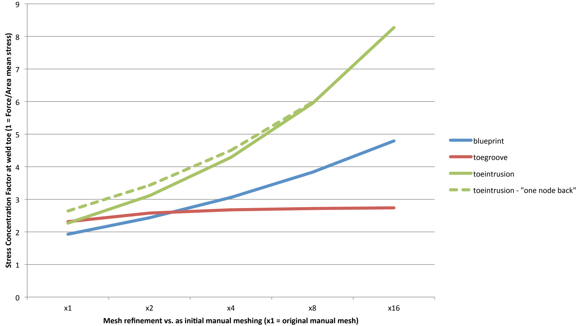
Finite Element Analysis outcome - Fillet weld toe shapes
